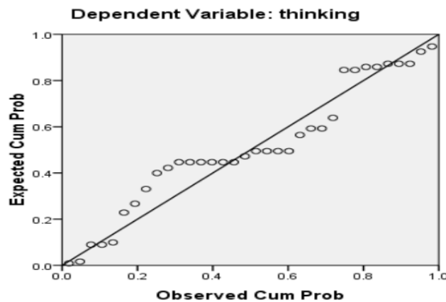
Fig 2. Normality test
